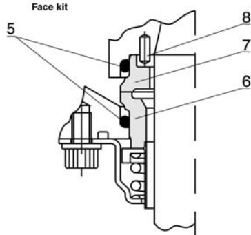
Face kit
