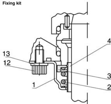
Fixing kit
