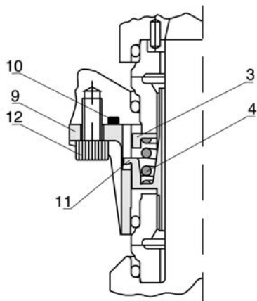
Fixing kit
