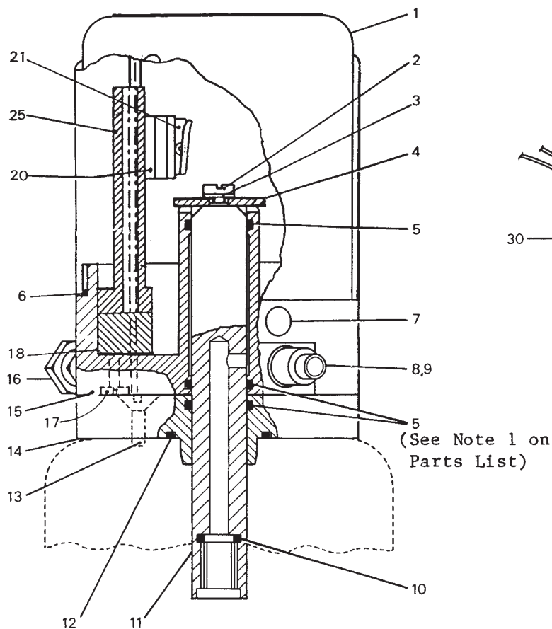
a) Sectional View (diagrammatic only)
