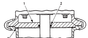
Mk1 (b) O-ring type shaft seal
