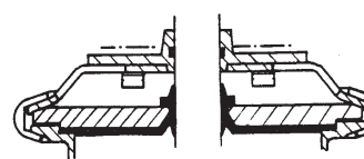
Mk2 (a) Lipseal type shaft seal
