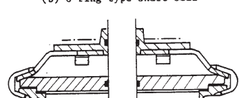
Mk2 (b) O-ring type shaft seal
